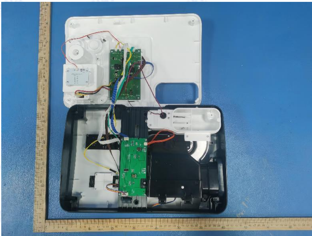
Photo 6: Internal view
